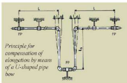
Principle for compensation of alterations in length by means of bending legs, related to length at angles
